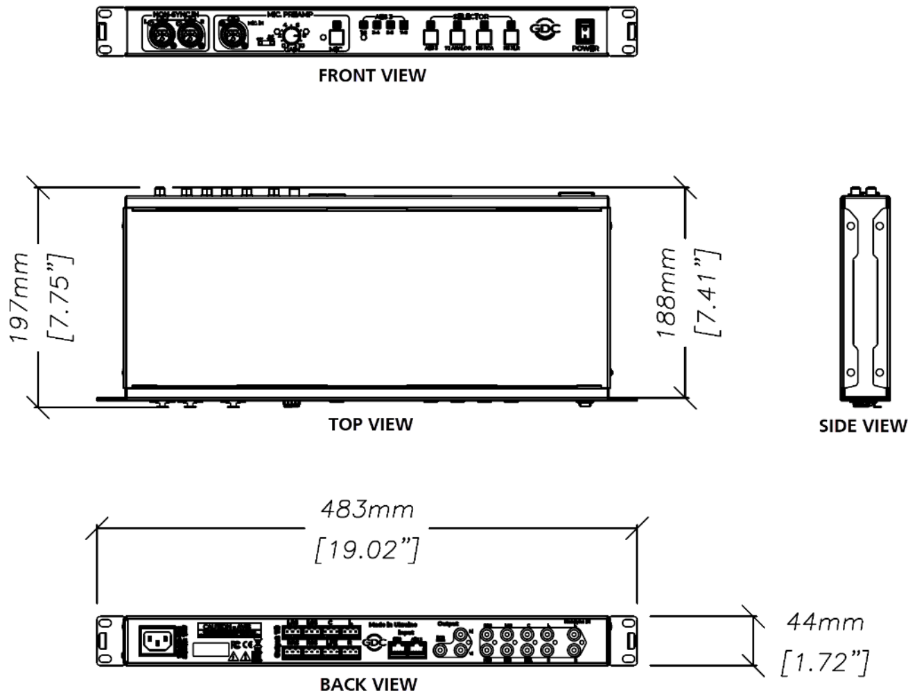
Figure 1: Dimensions of AIB-2000 Unit
